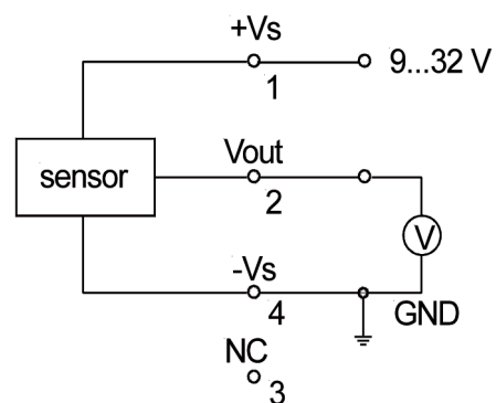
Electrical connection
